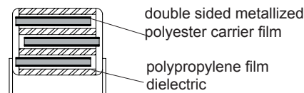
1 section (630Vdc/250Vac)
