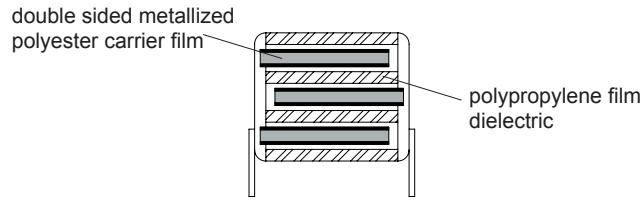
1 section (250Vdc)
